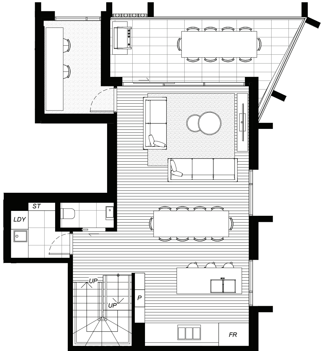
UPPER LEVEL 76 m 2
