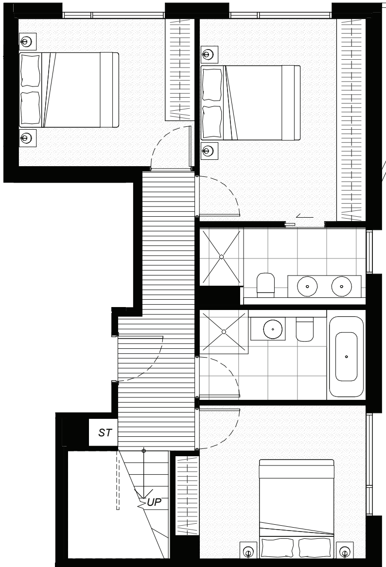
LOWER LEVEL 72 m 2 (ENTRY)
