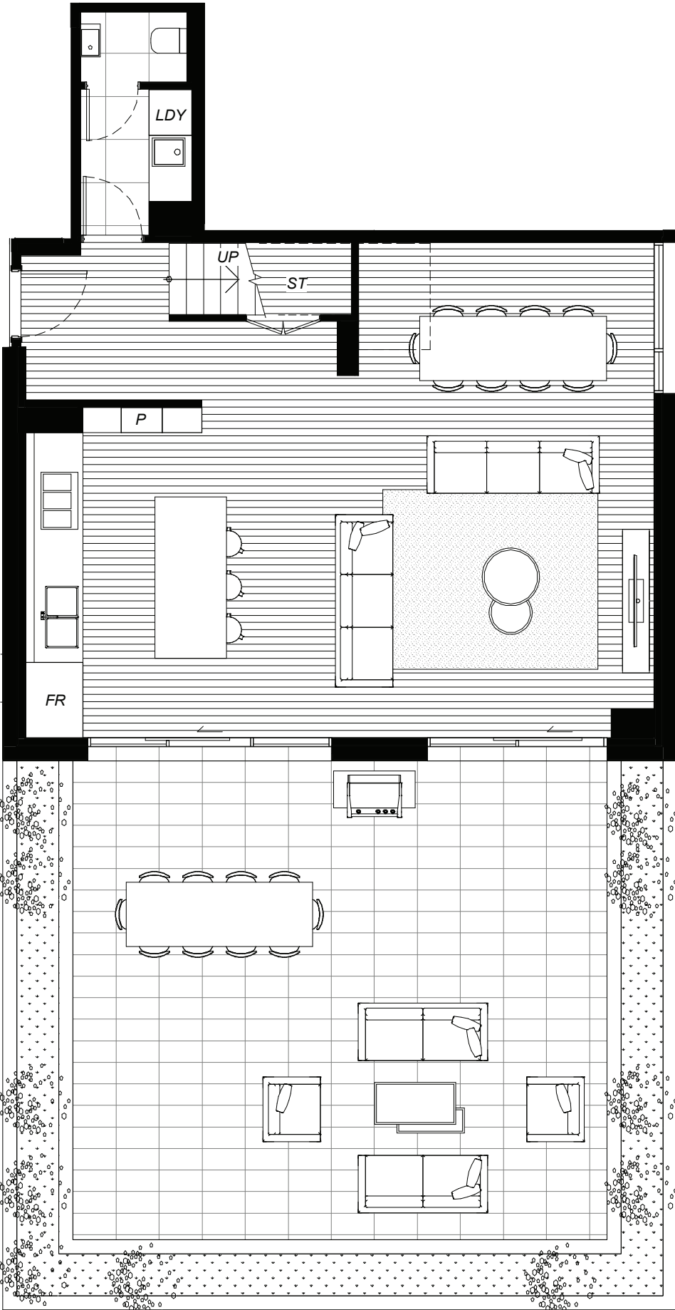
LOWER LEVEL 146 m 2 (ENTRY)
